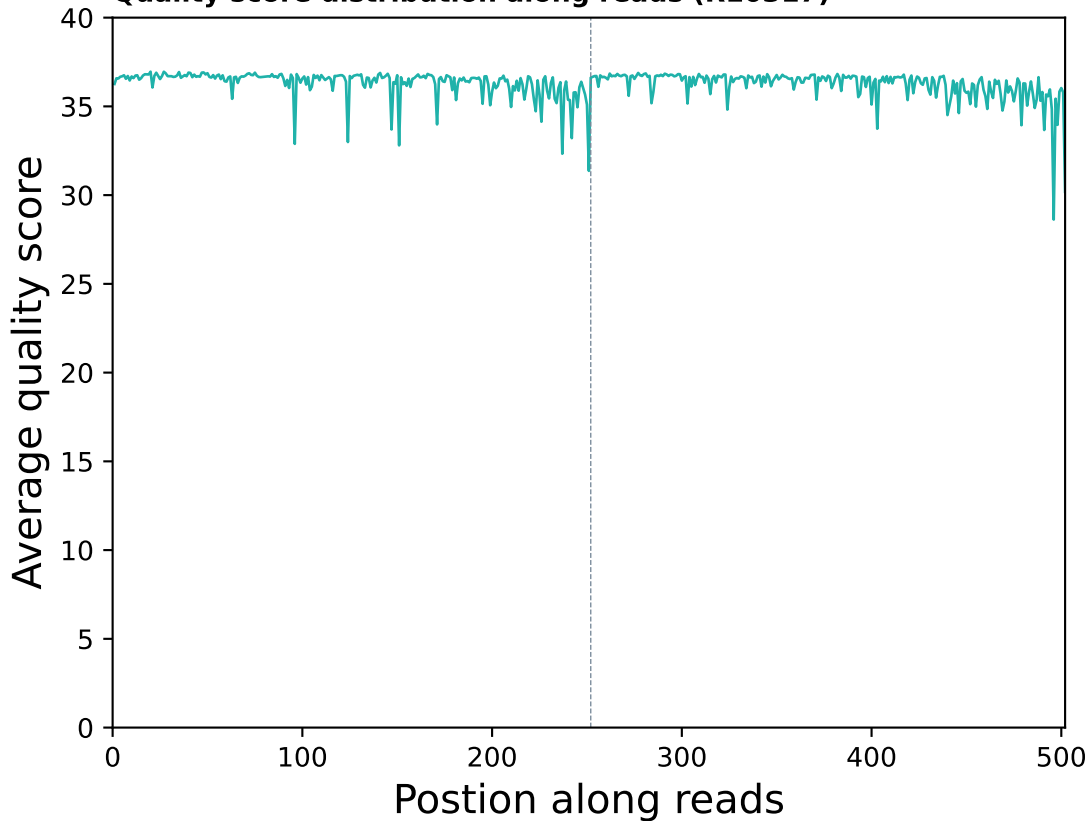
Quality score distribution along reads (R10317)
